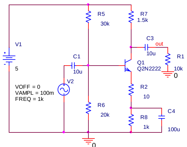
AC Sweep/Noise + Transient (THD)
