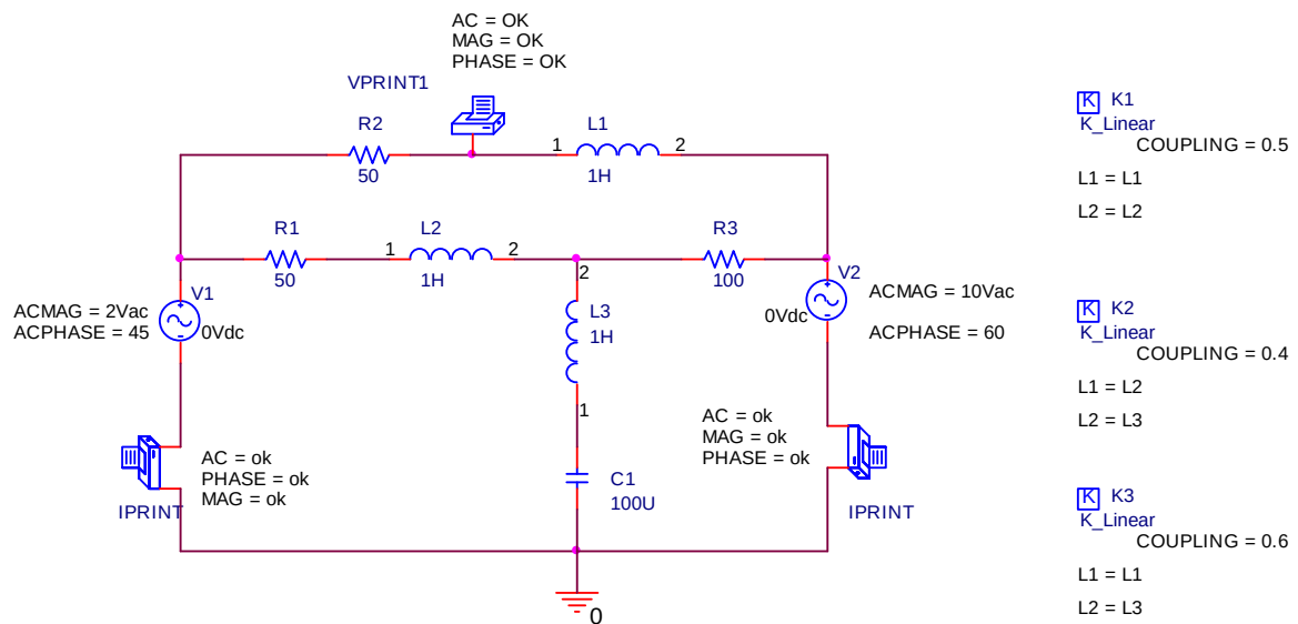
AC Sweep
