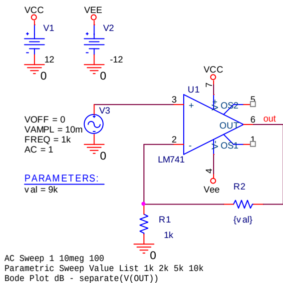
AC Sweep/Noise + Parametric Sweep
